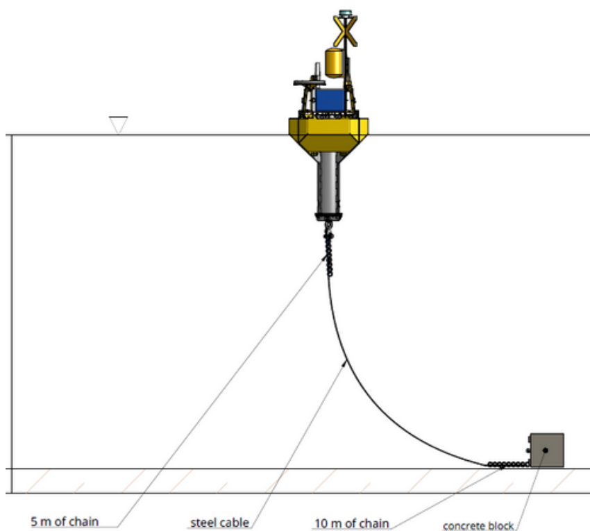
Drawing. 2 Buoy with anchoring system.
