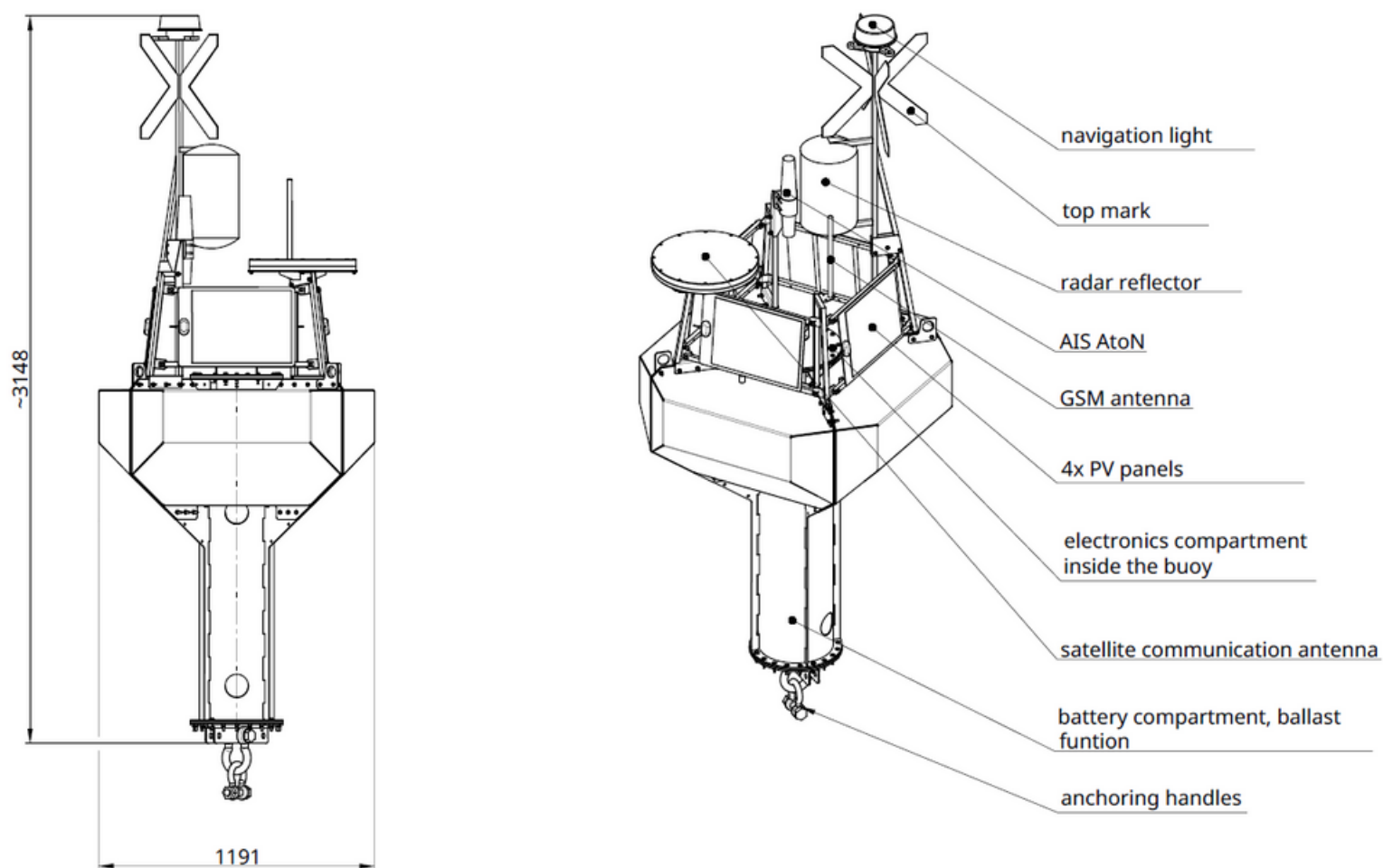
Drawing. 1 Dimensions and description of an example measurement buoy configuration.
